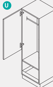
Garderobenschränk Höhe = 1907, 2051, 2195 mm Breite = 600 mm 2 feste Böden 1 Kleiderstange 1 Innenschubkasten Wardrobe unit Height = 1907, 2051, 2195 mm Width = 600 mm 2 fixed shelves 1 clothes rail 1 internal drawer
