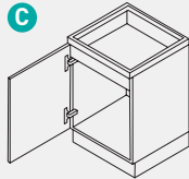
Spülenschränk Höhe = 723 mm Breite = 400, 450, 500, 600 mm 1 Drehtür Kitchen sink cabinet Height = 723 mm Width = 400, 450, 500, 600 mm 1 swing door
